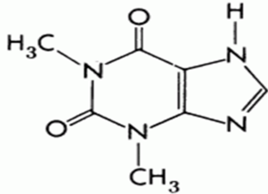
THEOPHYLLINE
